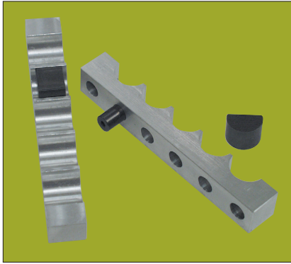
■ SGC404 Set of 2 aluminum pads for clamping aluminum cylinder heads (commonly used with SGC212).
