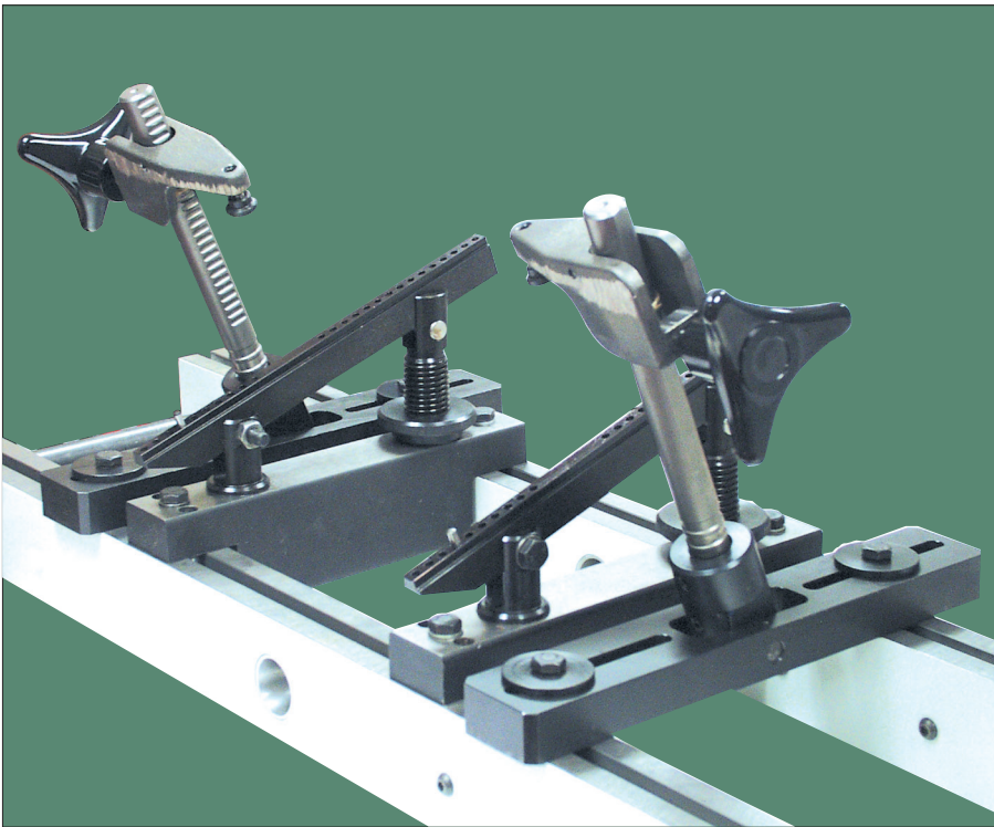
■ SGC212 Multi-angle cylinder head clamping fixture and set of 2 side clamps (SGC704 & SGC705 included).
